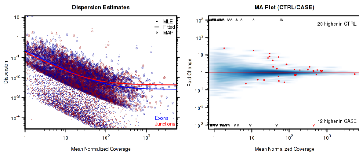
Figure 1: Summary Plots
