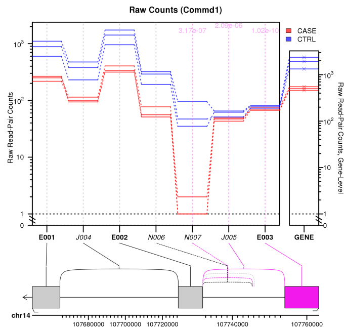
Figure 10: Raw counts for each sample
