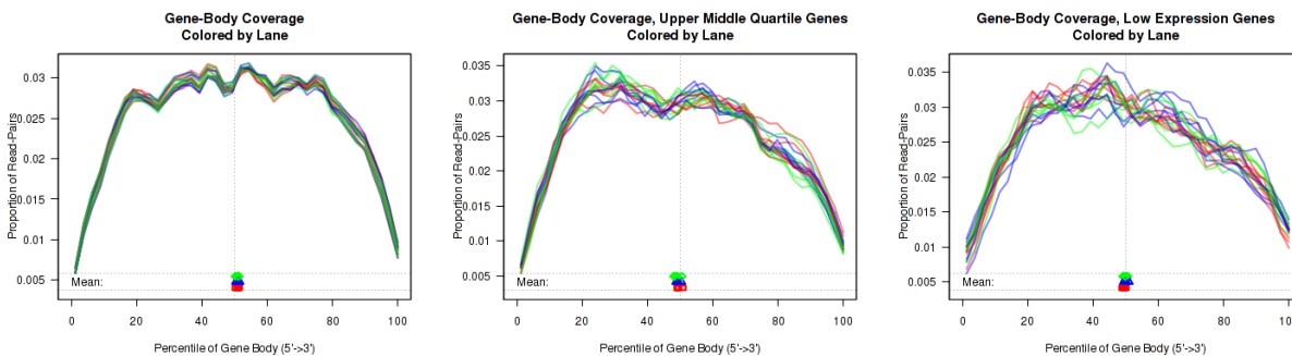
Figure 15: Gene-Body Coverage
